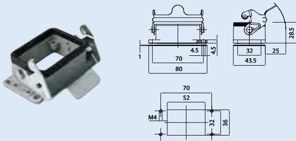
16x16A - 6x35A - 4/0x80A/16A - 4/2x80A/16A Makine Gövde
